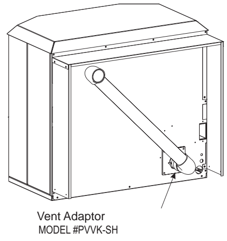
Figure 18 Single Flue - Venting with Shroud Installed Shroud Kit Model# PVSH
