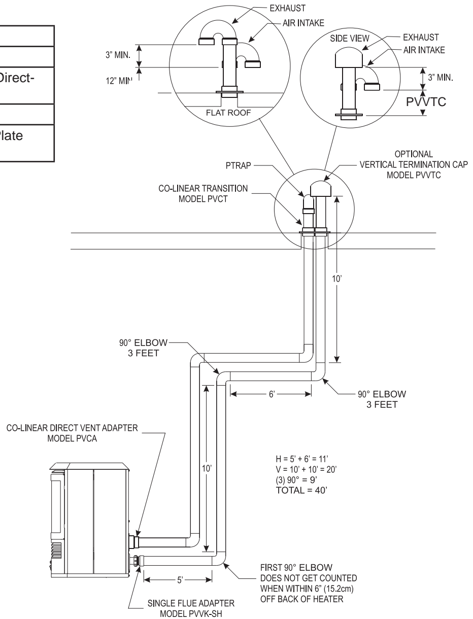
Figure 24 Calculation example of vent run maximum 40'
