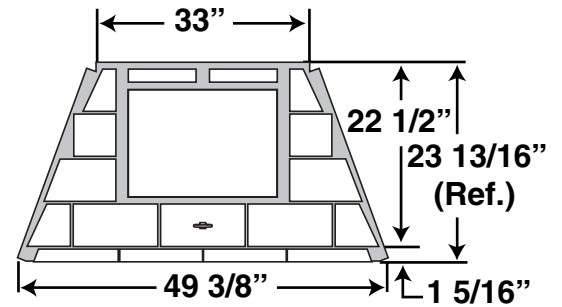
Hearth Dimensions
